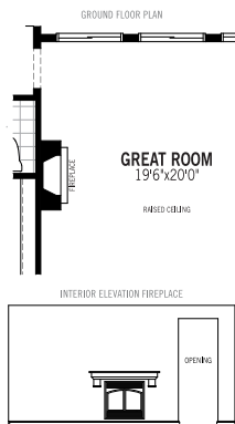
1 FIREPLACE AT GREAT ROOM
