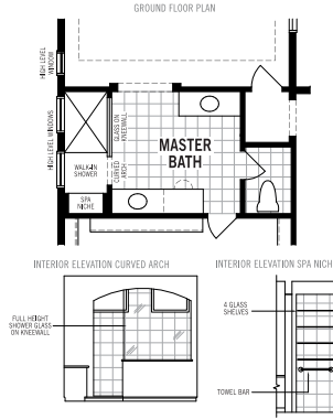
7 WALK-IN SHOWER W/SPA NICHE
