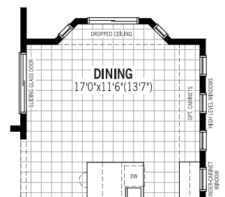
4 BAY WINDOW AT DINING (ADDITIONAL 19 SQ.FT.)
