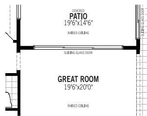
3 15' SLIDING GLASS DOOR AT GREAT ROOM
