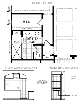
12 WALK-IN SHOWER W/SPA NICHE
