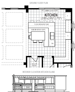
9 KITCHEN ISLAND W/BUILT-IN SEATING
