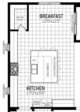
2 GOURMET KITCHEN
