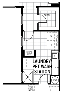
6 EXTENDED LAUNDRY W/PET GROOMING STATION IN LIEU OF GARAGE STORAGE
